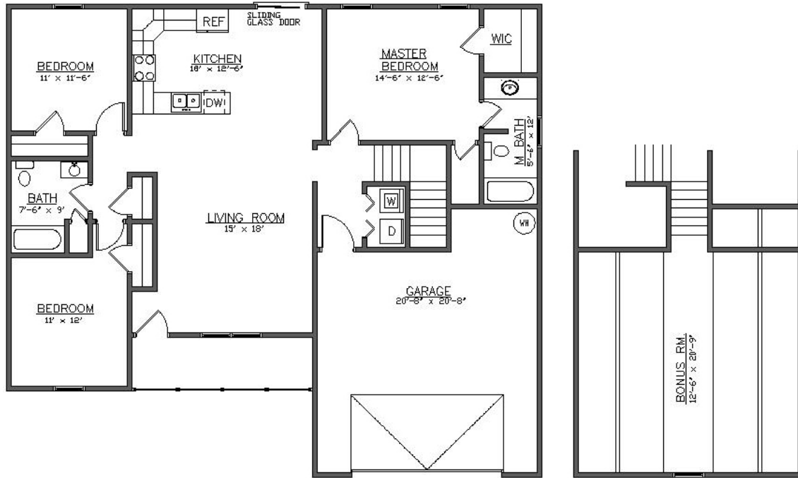
The Saluda with Bonus Floor Plan 1700 Sq. Feet
