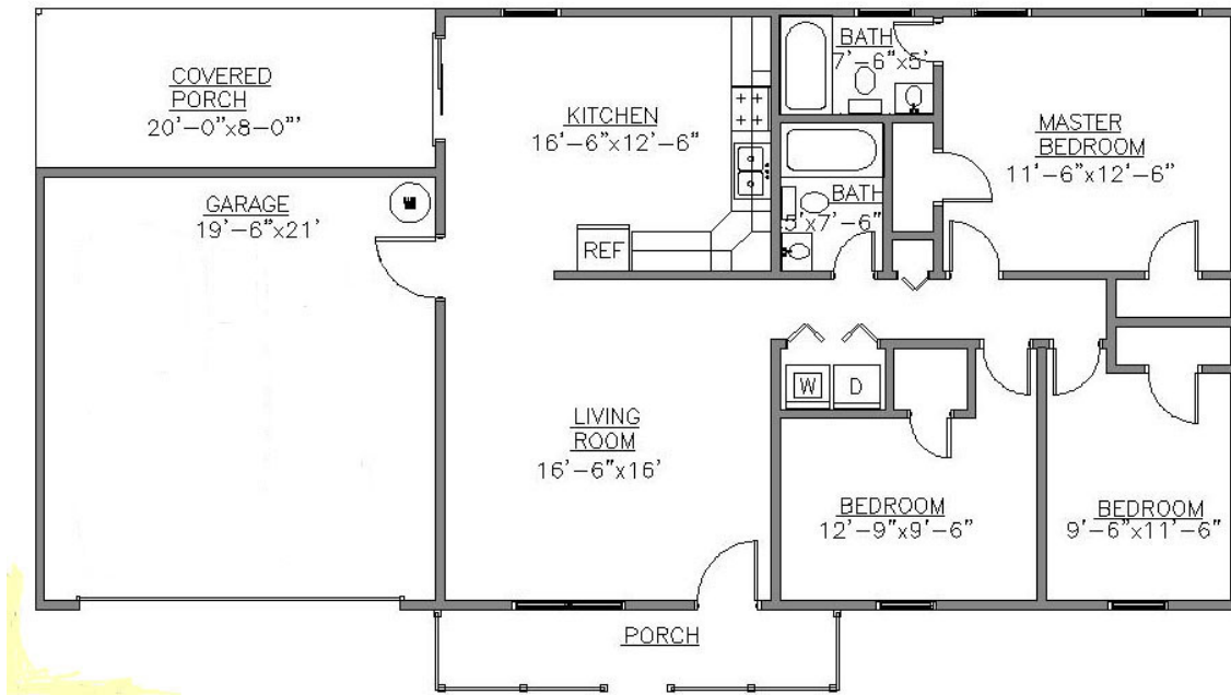
The Ashley Floor Plan 1200 Sq. Feet
