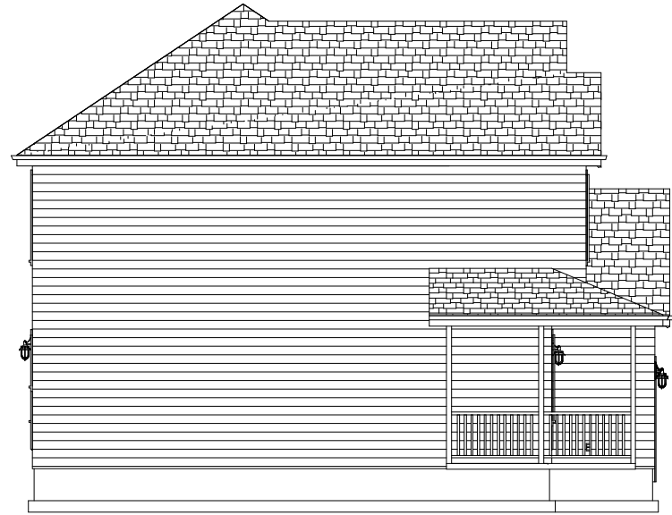
Left Elevation
