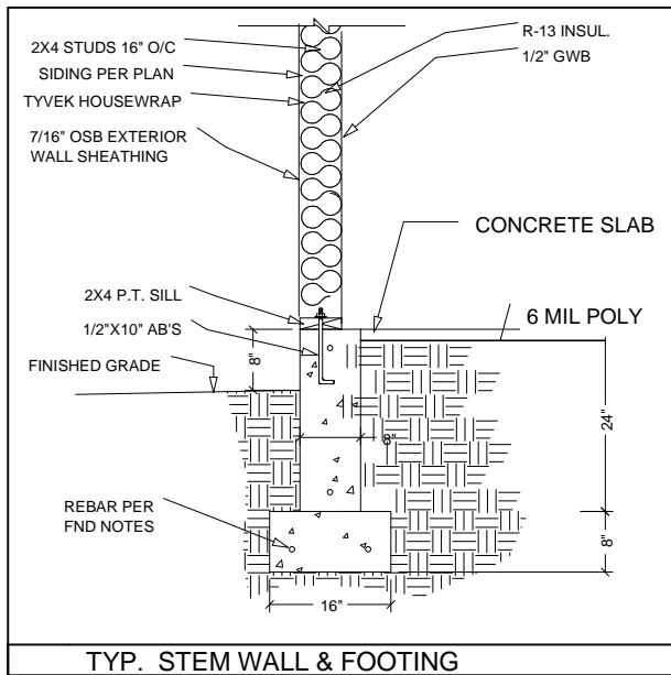
TYP. STEM WALL & FOOTING
